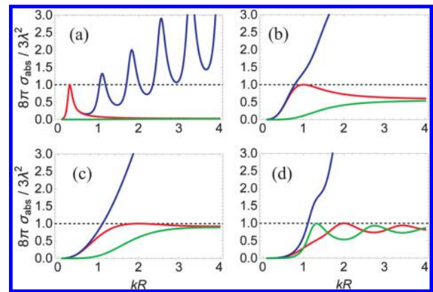
Figure 3. Dimensionless absorption cross sections, 8\pi\sigma_{\text{abs}}/(3\lambda^2) , plotted as a function of kR for IA designed to occur at: (a) kR = 0.3 , \bar{\epsilon}_s = -2.21 + i0.0611 ; (b) kR = 1 , \bar{\epsilon}_s = -1.87 + i2.91 ; (c) kR = 2 , \bar{\epsilon}_s = 0.4809 + i1.148 ; and (d) kR = 2 , \bar{\epsilon}_s = 4.968 + i1.361 . Total absorption cross sections are given by blue curves, electric dipole absorption by red curves, and magnetic dipole absorption by green curves.
