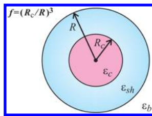
Figure 6. Schematic of a concentric coated sphere where the core, shell, and background permittivities are denoted, respectively, \epsilon_c , \epsilon_{sh} , and \epsilon_b . The filling fraction of the core material is defined as f \equiv (R_c/R)^3 .
