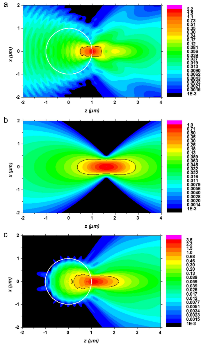
Fig. 1. (a) Total electric field intensity map in logarithmic scale for d = 1.62 \mu\text{m} . The white circle represents the microsphere section, the thin black line represents the I_{max}/e^2 intensity contour. (b) and (c) display the intensity maps of the incident and scattered fields. The coherent summation of these two fields leads to the total intensity presented in (a).
