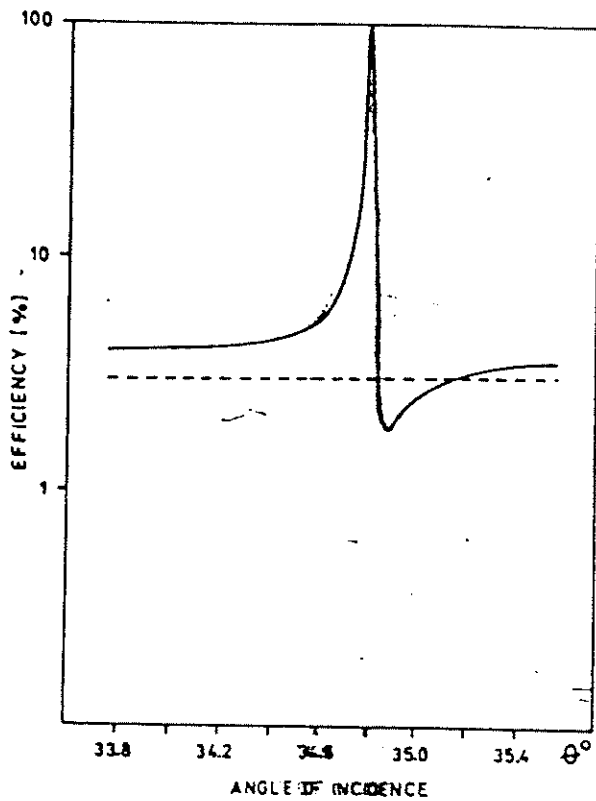
Fig. 1. Calculated reflected zero-order efficiency of sinusoidal grating as a function of the angle of incidence; the parameters are given in the text. Dashed line: bare dielectric grating, solid line: coated grating.
