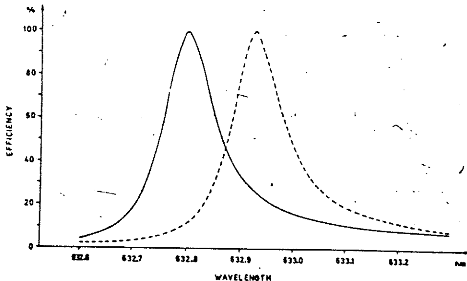
Fig. 2. Theoretical zero-order reflectance as a function of the wavelength. Solid line: angle of incidence 34.77^\circ , with maximum wavelength 632.8 \text{ nm} ; dashed line: angle of incidence 34.80^\circ .
