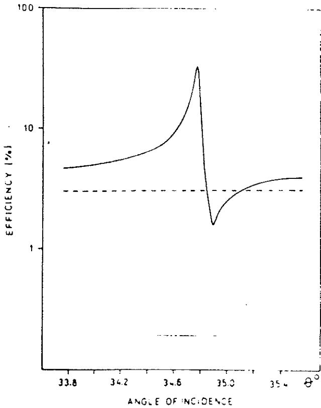
Fig. 3. Measured zero-order reflection efficiency as a function of the angle of incidence; the grating parameters are given in the text. Dashed line: before ion-exchange. Solid line: after formation of the waveguide.
