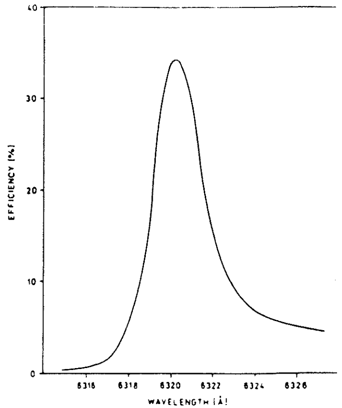
Fig. 5. Experimental wavelength dependence of the zeroth-reflecting order efficiency.
