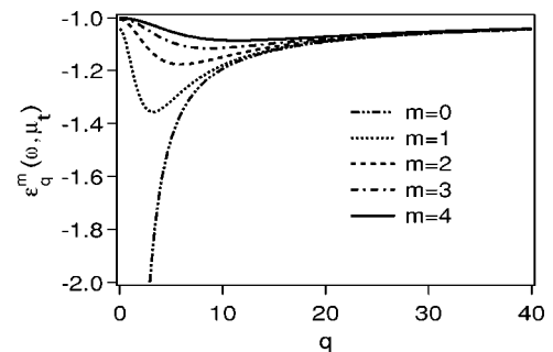
FIG. 3. The various azimuthal modes m of a probe with \theta_i = 30^\circ . As shown, in the limit m \rightarrow \infty , the modes approach the surface plasmon dispersion of a vacuum-bounded metal half space for all q . All modes reach their asymptotic values for q \gtrsim 20 .
