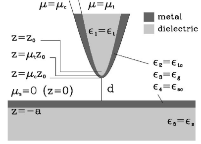
FIG. 1. Geometric representation of a metal-coated dielectric probe above a metal-coated dielectric substrate in spheroidal system in the \varphi=0, \pi planes, where \varphi is the azimuthal coordinate. The probe tip boundary is defined by \mu_t = \cos \theta , where the angle \theta is measured from the symmetry axis of the hyperboloid ( z -axis) to an asymptote to the hyperboloid. The surface of the coating is given by \mu_c . The boundary of the substrate metal coating ( z=0 plane) is set by the hyperboloid \mu_s = \cos \theta_s with \theta_s = \pi/2 , while that of the substrate is defined by z=-a . The dielectric functions characterizing the involved materials in the five regions are labeled by \epsilon_1 through \epsilon_5 defined in the figure.
