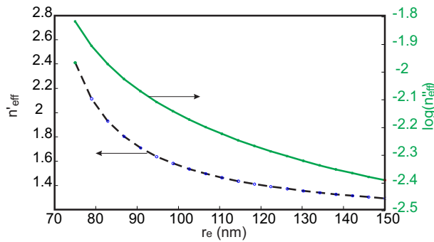
Figure 9.19: Real part n_{eff}^l and \log_{10} of the imaginary part n_{eff}^r of the effective index associated with the TEM-like mode of an infinite coaxial waveguide as a function of the outer radius r_e . The inner radius is set to r_i = 65 nm and the working wavelength is \lambda = 1550 nm.
