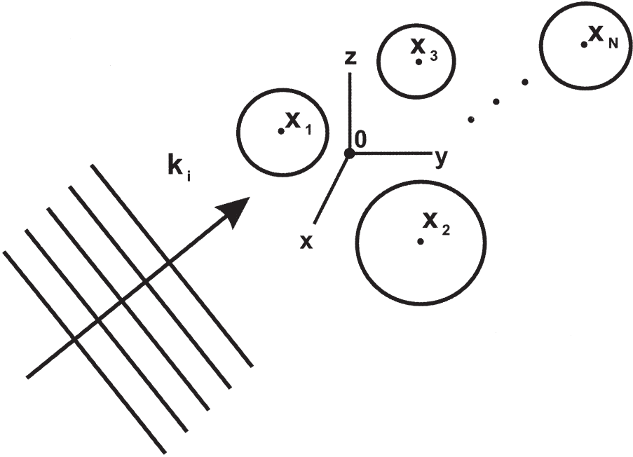
Figure 1. A two-dimensional projection of a system of multiple light scattering by spheres. A field is incident on the system with a wave-vector \mathbf{k}_i . The centres of the spheres are denoted \mathbf{x}_j , j = 1, \dots, N , N being the number of spheres in the system.
