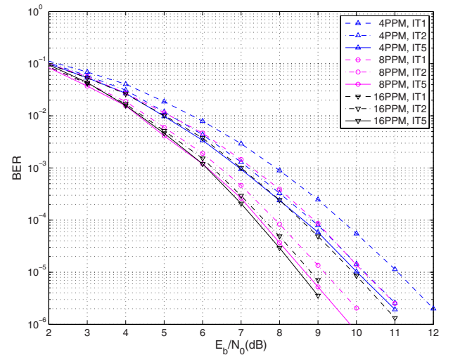
Fig. 5. (Color online) Performance of the iterative receiver for the weak turbulence channel with \chi^2 = 0.04 , Q -ary PPM with Q = 4, 8, 16 , RSC (1,5/7) code; IT m denotes the m th iteration.
