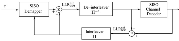
Fig. 2. Block diagram of the iterative receiver. \text{LLR}_{\text{DEM}}^{\text{ext}} and \text{LLR}_{\text{DEC}}^{\text{ext}} , extrinsic soft values at the demapper and the channel decoder, respectively.
