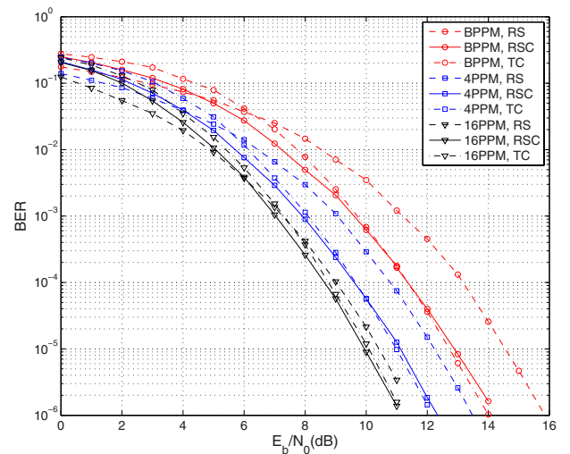
Fig. 3. (Color online) Comparison of different coding and modulation schemes, weak turbulence regime with \chi^2=0.04 . RSC code, (1, 5/7); RS code, (239, 255); TC, punctured parallel concatenation of two RSC (1, 5/7) codes.
