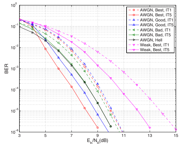
Fig. 7. (Color online) Performance of the iterative receiver for 2-4PPM modulation with B=2 for different mappings for the AWGN channel and the “Best” mapping for the weak turbulence channel. RSC (1,5/7) code; IT m denotes the m th iteration.
